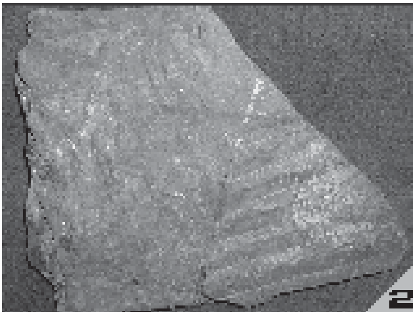
Plan o a IV. Cladophlebis silvaeregis Czier. 1. MPCO-STN 6551/2. 2. MPCO-STN 8996.
