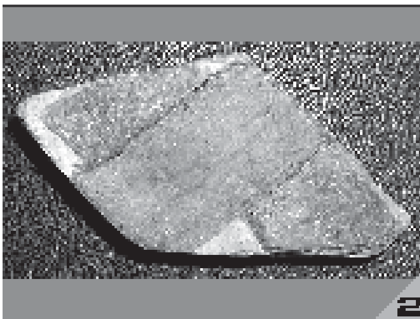
Plan o VIII. Receaphyllum grandis Czier. 1. M PCO -STN 16502. 2. M PCO -STN 16504.
