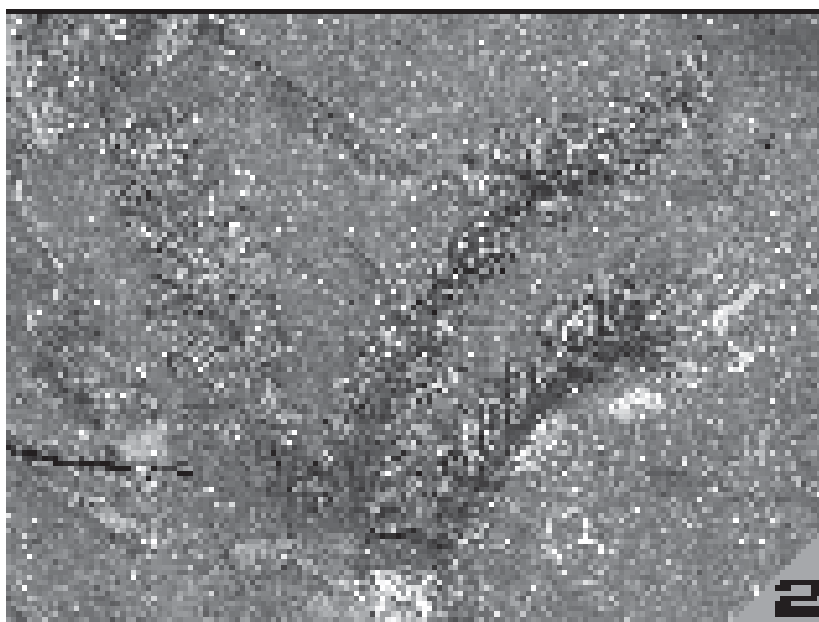
Plan o a V. Selenocarpus muensterianus (Presl in Sternberg) Schenk. 1. MPCO-STN 6549/A. 2. MPCO-STN 6549/B.
