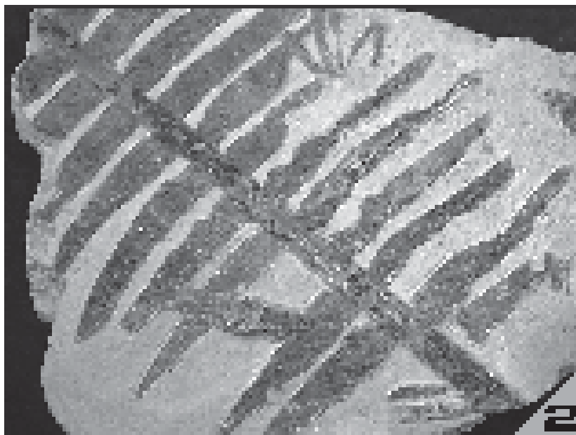
Plan o a VII. 1. Selenocarpus muensterianus (Presl in Sternberg) Schenk. MPCO-STN 6550. 2. Receaphyllum grandis Czies. MPCO-STN 16501/1.
