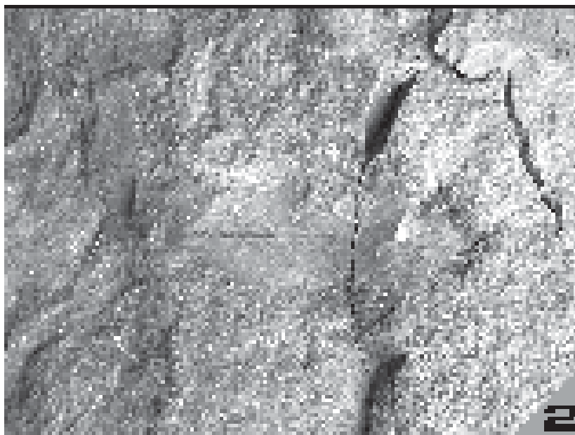
Plan o a I. 1. Cladophlebis obtusifolia (Andrae) Schimper in Ward. MPCO-STN 16527/1. 2. Cladophlebis indica (Oldham et Morris) Sahni et Rao. MPCO-STN 15332/2.
