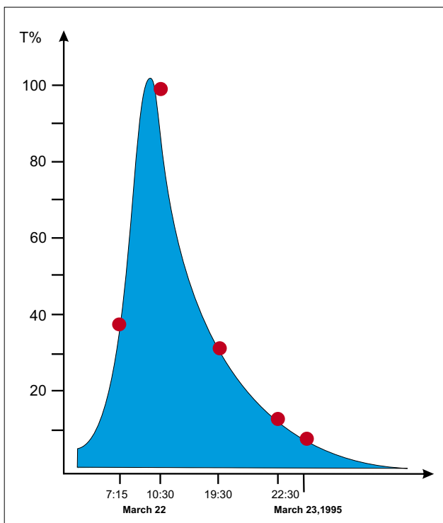
Figure 6. Graph of the tracer output at Izbucul cu Cascadă spring for the input in Cuciulata Pit, credit by Emil Silvestru, 1995
