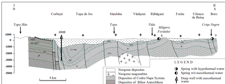
Figure 3. Cross section between Corbești – Borz. Line of section in Figure 2.
